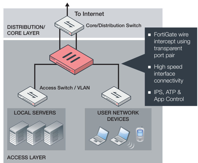
FIGURE 5 –INTERNAL SEGMENTATION FIREWALL (ISFW) DEPLOYMENT
